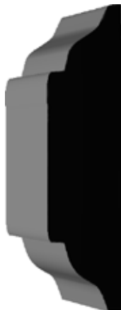
Chair rail TM224 300224 9/16 x 2-1/4 x 8', R/L
