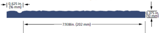
LP SmartSide Colonial Beaded Lap (smooth)
