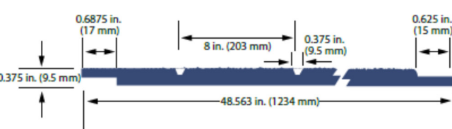
LP SmartSide 76 series Cedar Panel 8 in. O.C.
