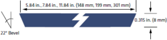
LP Smartside 38 Series Lap Siding
