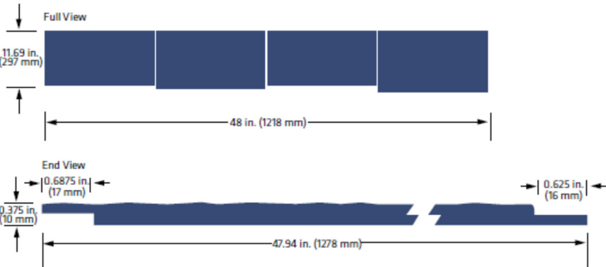
LP® SmartSide® Cedar Shakes
