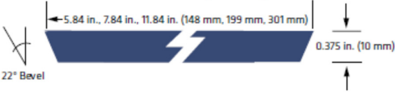
LP Smartside 76 Series SmartLock Lap Siding
