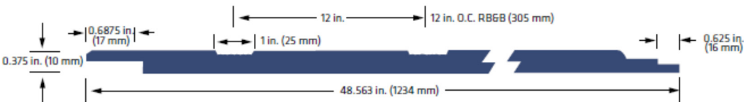
LP SmartSide Reverse Board and Batten Panel 12 In. O.C.
